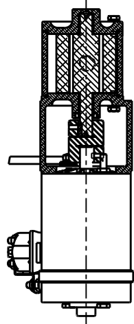
SECTION A-A SCALE 1/2
