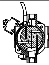
SECTION B-B SCALE 1/2
